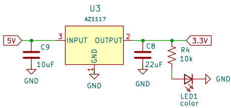
Voltage Regulator 5V -> 3.3V
