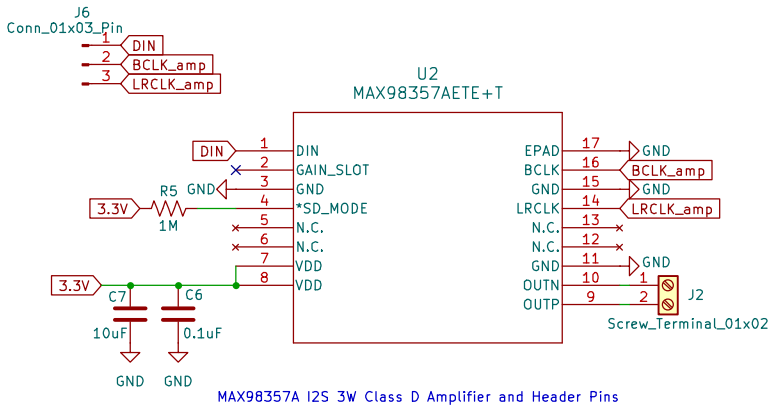
MAX98357A I2S 3W Class D Amplifier and Header Pins
