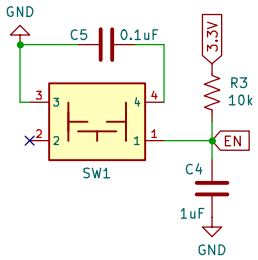
Restart Button: ESP32-S3-WROOM-1 Restart on Press
