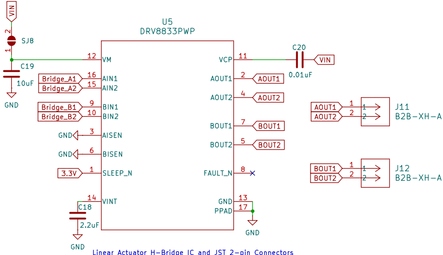
Linear Actuator H-Bridge IC and JST 2-pin Connectors
