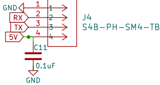
UART Nexion Display JST 4-pin Connector (side)
