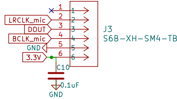
Adafruit SPH0645LM4H JST 6-pin Connector (side)
