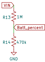
Battery Percentage Circuit
