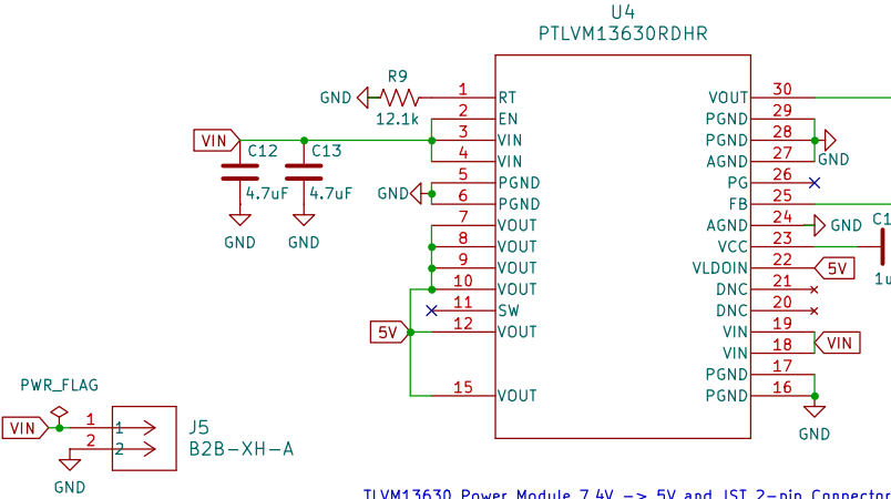
TLV13630 Power Module 7.4V -> 5V and JST 2-pin Connector
