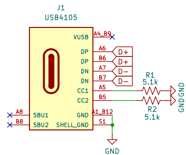
USB-C Connector: 5V Power and ESP32-S3-WROOM-1 Programming
