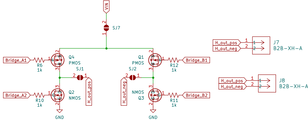
Linear Actuator FET H-Bridge and JST 2-pin Connectors
