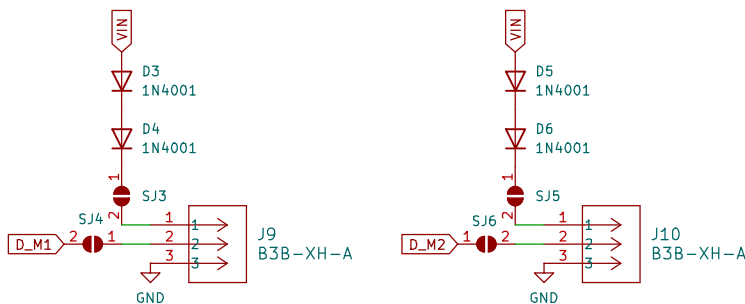
Motors and JST 3-pin Connectors
