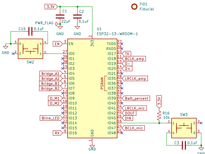
ESP32-S3-WROOM-1 Boot-Mode Button and Pin-outs
